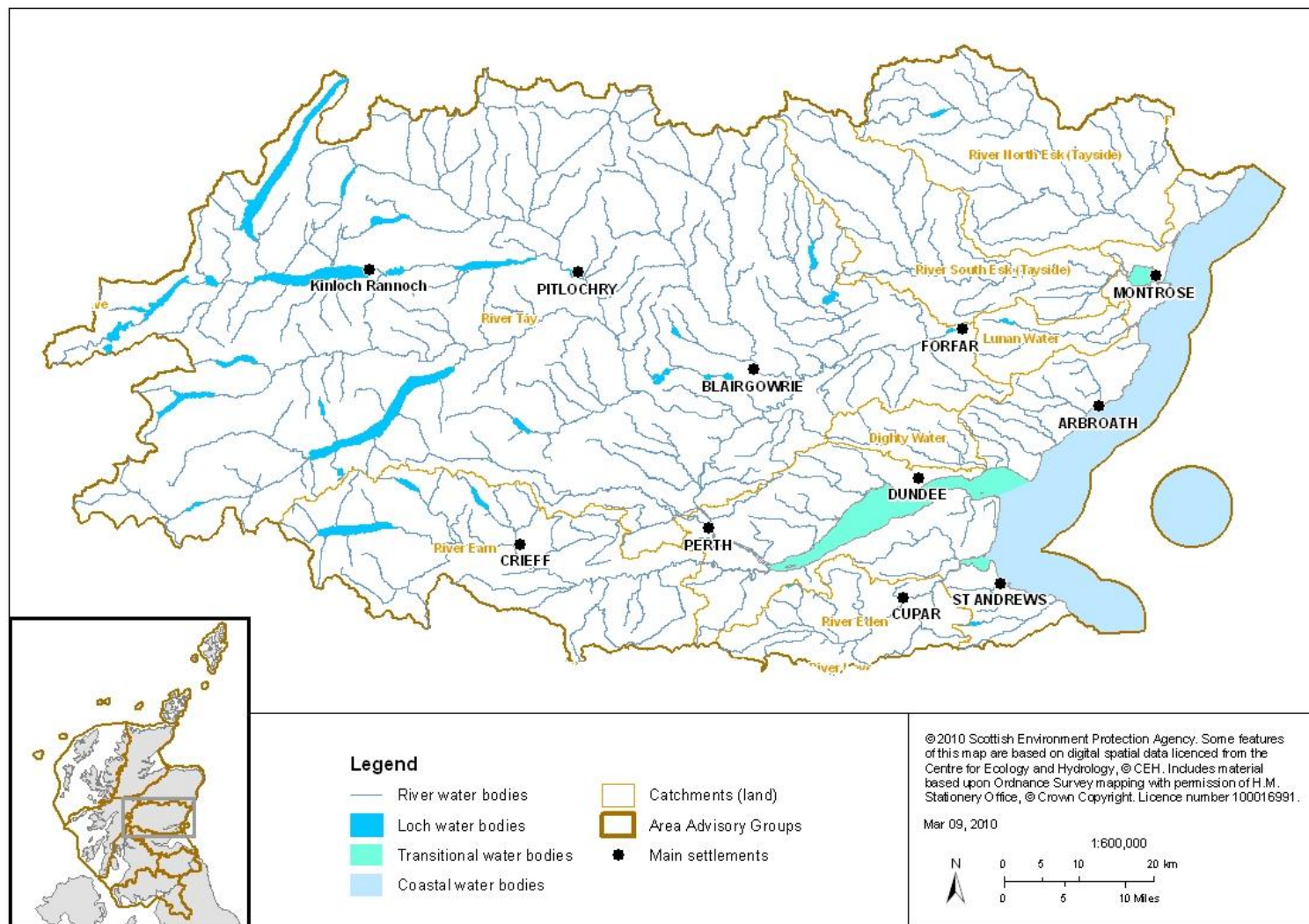
Map 1: Tay advisory group area (showing main river catchments)
