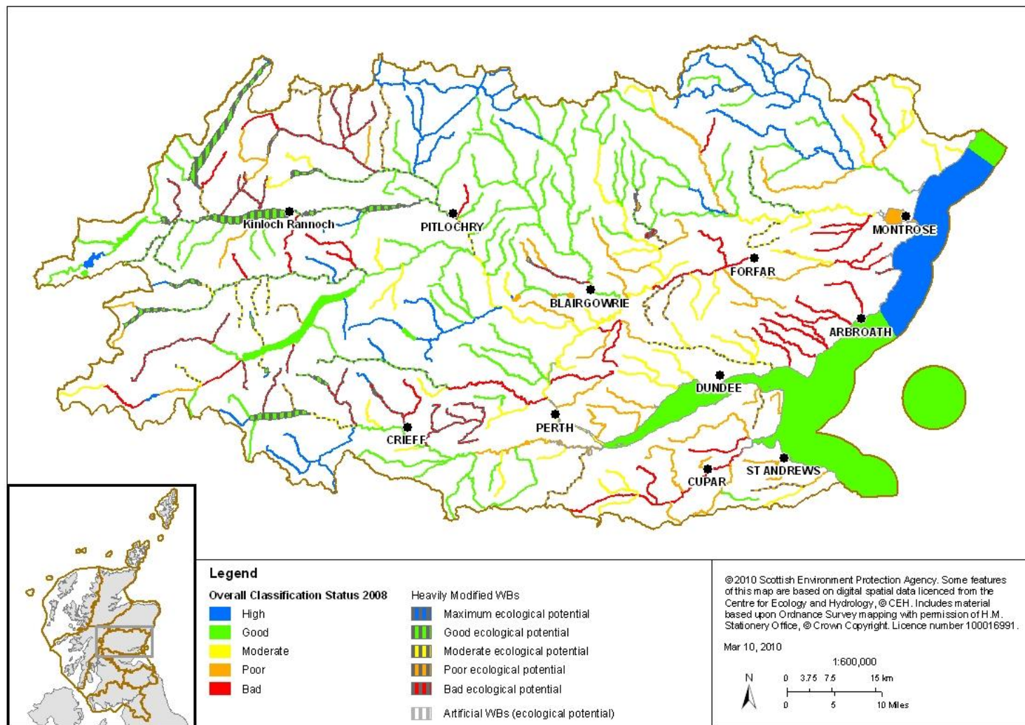
Map 2a: Current condition of surface and coastal water bodies in the Tay advisory group area
