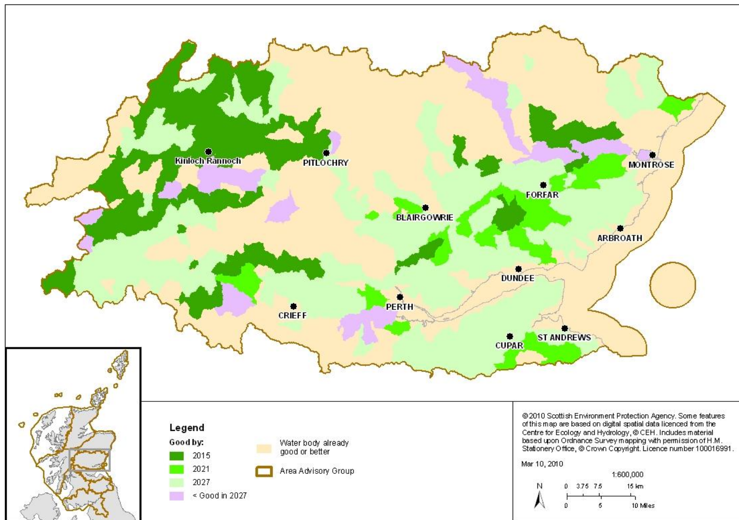
Map 3: Planned improvements for surface waters, 2015–2027
