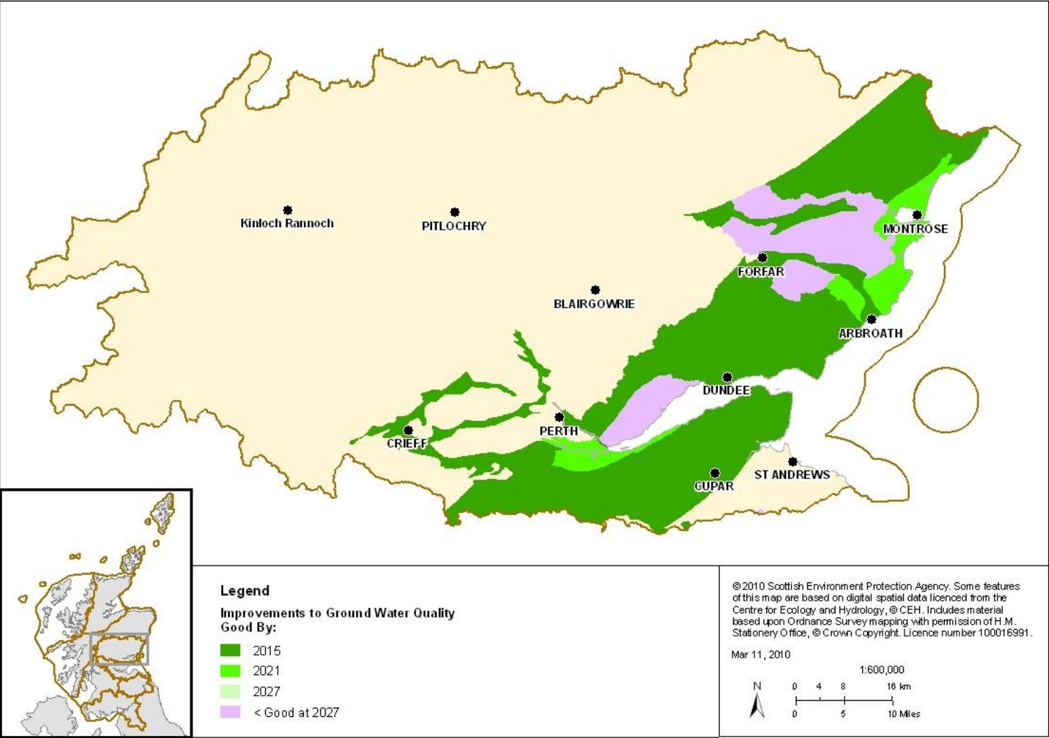
Map 4: Planned improvements for groundwaters, 2015–2027
